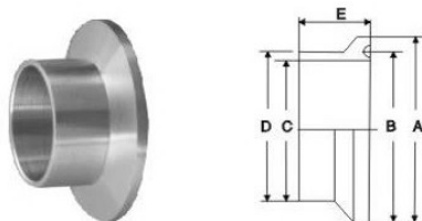
卫生级快装接头 Fast joint health level
