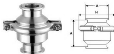
卫生级快装止回阀 Sanitary quick install check valve
