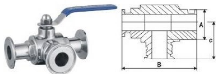
卫生级快装三通球阀 Sanitary quick install three ball valves
