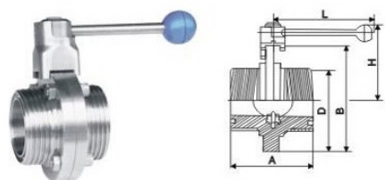
卫生级螺纹蝶阀 Hygienic thread butterfly valve
