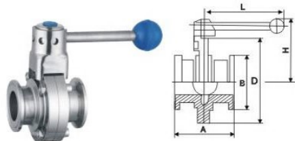
卫生级快装蝶阀 Sanitary quick butterfly
