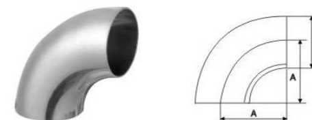
卫生级焊接式90°弯头 Sanitary welding type elbow 90°
