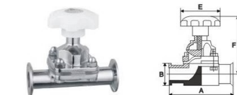
卫生级隔膜阀 Sanitary diaphragm valve
