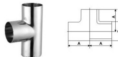
卫生级焊接式三通 Sanitary welding type three
