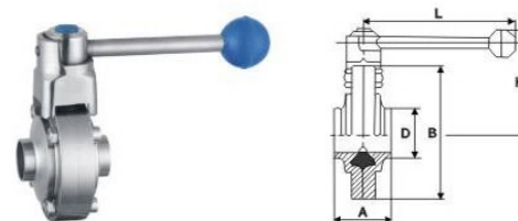
卫生级焊接式蝶阀 Sanitary welding type butterfly valve
