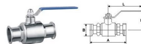
卫生级球阀 Sanitary ball valve
